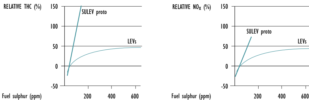
Figure G-5: Effects of Fuel Sulphur on Emissions (relative to 30 ppm Sulphur Fuels)
